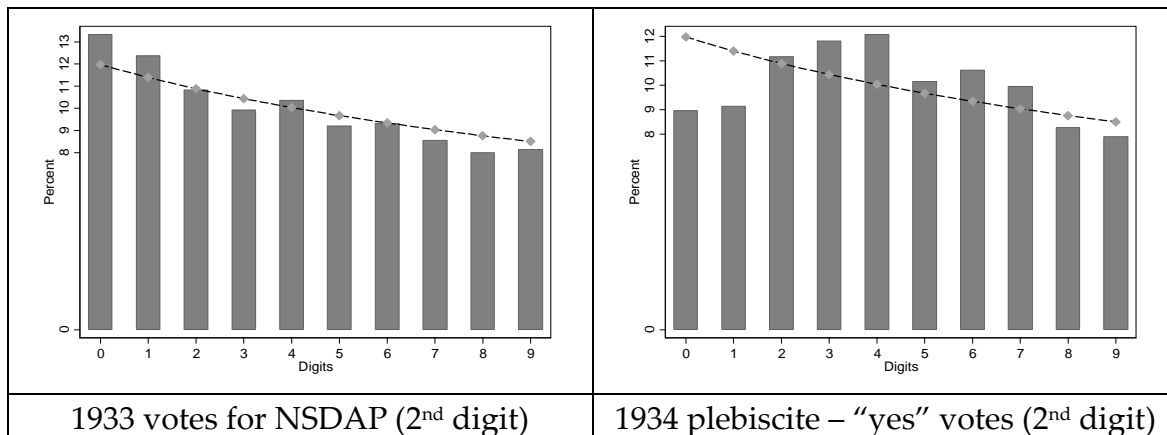
Figure 5: Benford’s Law – predicted vs actual values [dotted line vs bars]
